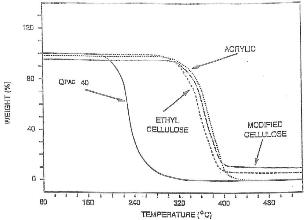
Figure 1. TGA Results of Various Binders in Nitrogen
